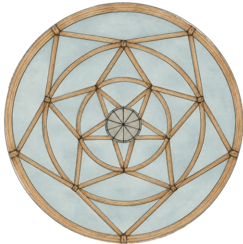
ROUND BARN GREENHOUSE ELEVATION & ROOF PLAN
