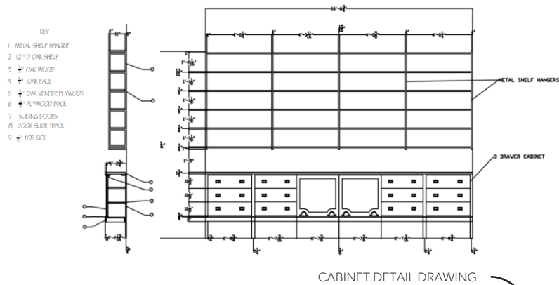
CABINET DETAIL DRAWING
